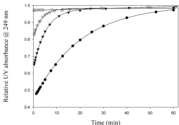
Figure 3. Kinetic study on the cyclization processes: Measuring UV absorbance at 249 nm of the filtrates from 4 min's hydrogenation of compounds 1a (●), 1b (○), 1c (▼), and 1d (▽) against time: expressed in the ratio of absorbance at certain time interval versus absorbance at T=120 min when the absorbance for each compound has reached a constant.
