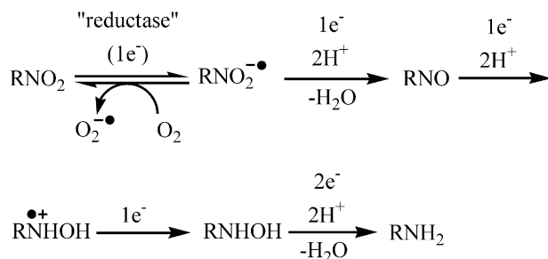
Figure 1. Selectivity of nitroaromatics towards hypoxia.
