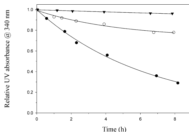
Figure 4. Stability of NADH under different incubating conditions. Relative UV absorbance of NADH against time: expressed by the ratio of the absorbance at certain time interval versus absorbance at time zero for each incubating condition. The conditions used were 100 mM phosphate buffer at 37°C (●), 10 mM phosphate buffer at 37°C (○), and 10 mM phosphate buffer at 25°C (▼).
