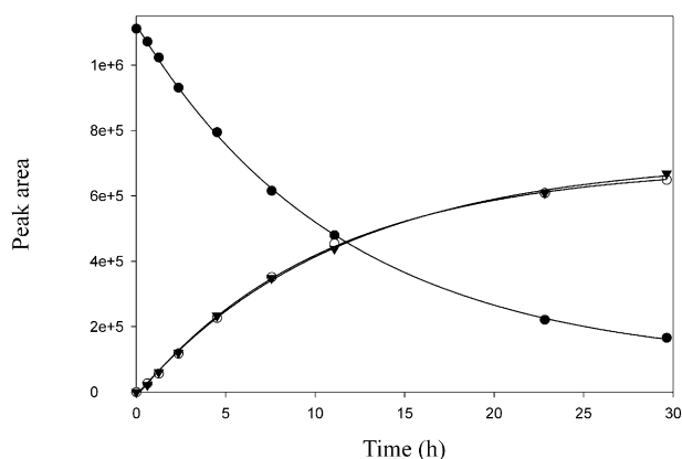
Figure 5. Reduction of compound 1c by E. coli B nitroreductase: Composition of a solution of 1c reductively activated by nitroreductase against time. Shown are the disappearance of 1c (●) and appearance of 4c (○) and FUDR (▼).
