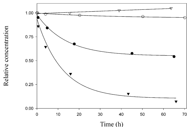
Figure 2. Stability of compounds 1a (●), 1b (○), 1c (▼), and 1d (▽) in human serum. Relative concentration against time: expressed by the ratio of the peak area at certain time interval versus peak area at time zero for each compound.
